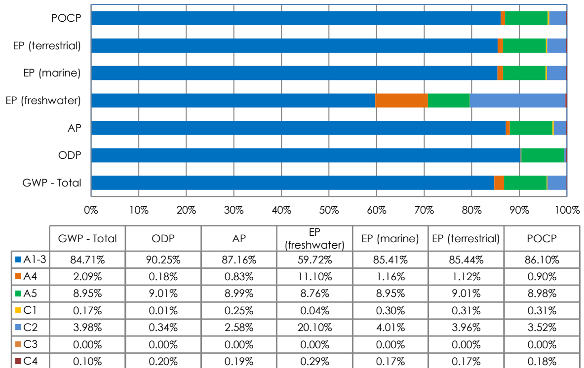
Figure 1 - shows the relative contribution of each life cycle stage to different environmental indicators for the carbon steel reinforcing bar products manufactured by the secondary (scrap based) production route
